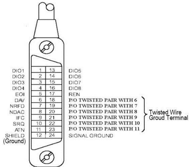
GPIB Cable Connection Method 1:
